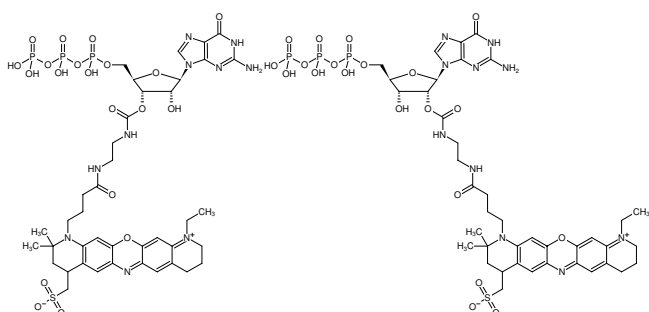
Structural formula of EDA-GTP-ATTO-655
