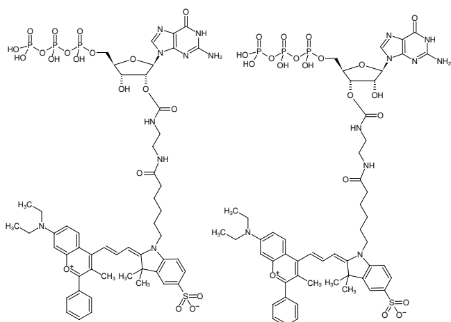
Structural formula of EDA-GTP-DYQ-660
