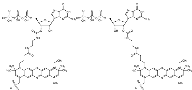
Structural formula of EDA-GTP-ATTO-700
