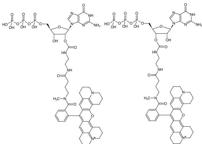
Structural formula of EDA-GTP-ATTO-Rho101
