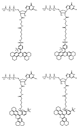
Structural formula of EDA-GTP-Texas Red
