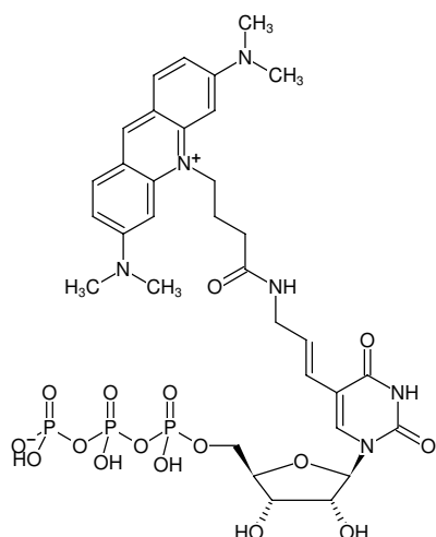
Structural formula of Aminoallyl-UTP-ATTO-495
