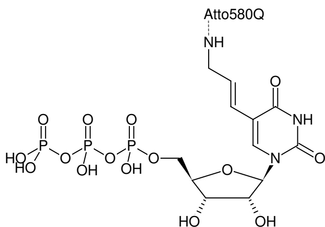
Structural formula of Aminoallyl-UTP-ATTO-580Q
