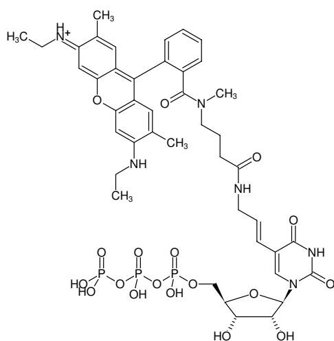
Structural formula of Aminoallyl-UTP-ATTO-Rho6G
