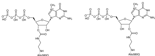
Structural formula of EDA-m 7 GTP-ATTO-580Q
