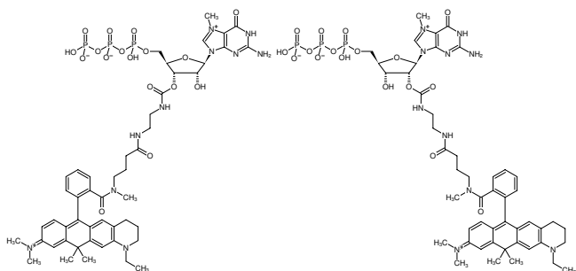
Structural formula of EDA-m 7 GTP-ATTO-633
