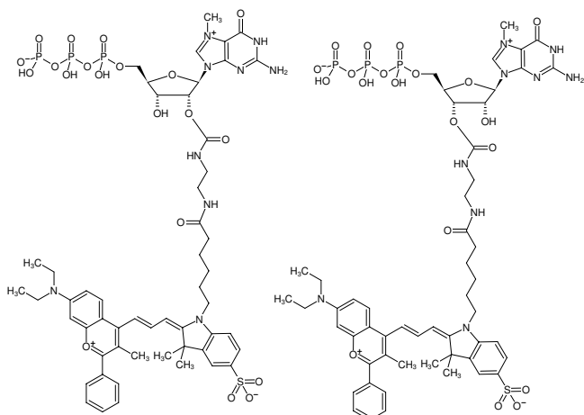
Structural formula of EDA-m 7 GTP-DYQ-660
