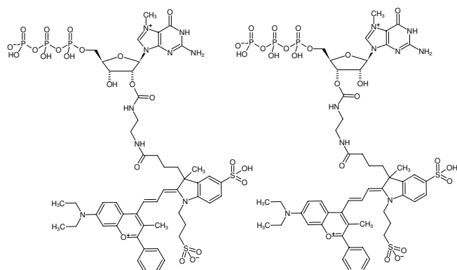
Structural formula of EDA-m 7 GTP-DYQ-661
