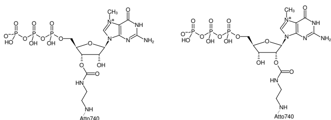
Structural formula of EDA-m 7 GTP-ATTO-740
