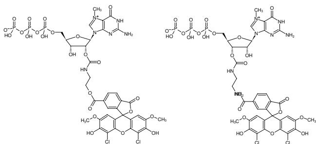
Structural formula of EDA-m 7 GTP-6-JOE
