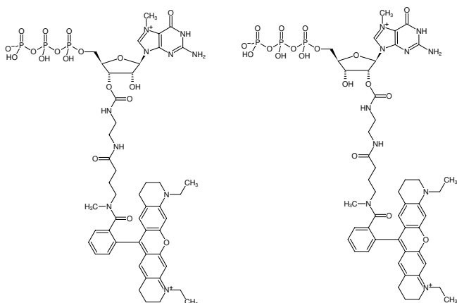
Structural formula of EDA-m 7 GTP-ATTO-Rho11
