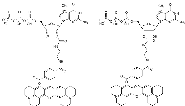
Structural formula of EDA-m 7 GTP-6-ROX
