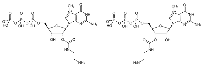
Structural formula of EDA-m 7 GTP
