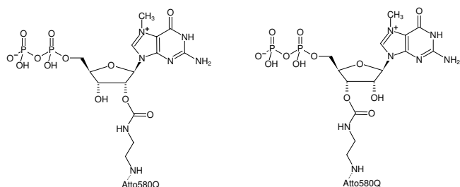
Structural formula of EDA-m 7 GDP-ATTO-580Q
