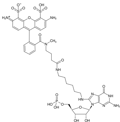
Structural formula of 8-(6-Aminoethyl)-amino-GMP-ATTO-488
