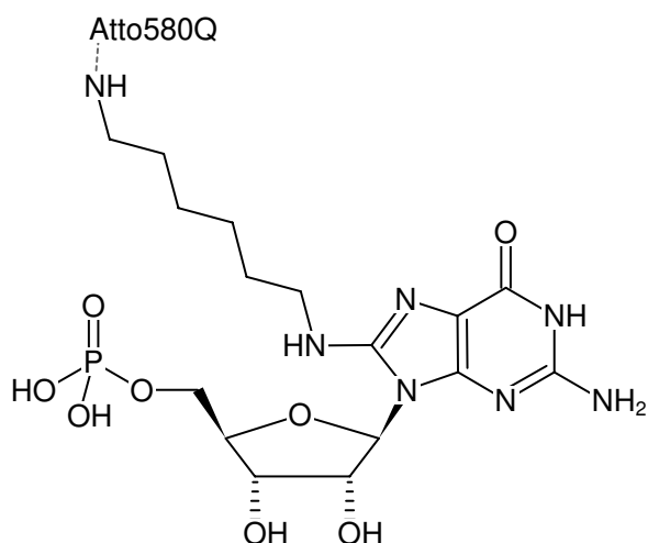
Structural formula of 8-(6-Aminoheptyl)-amino-GMP-ATTO-580Q
