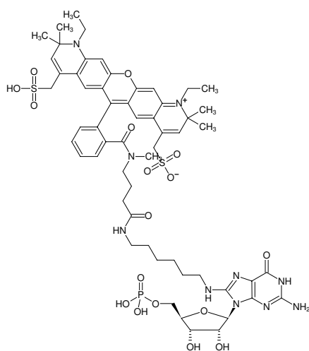
Structural formula of 8-(6-Aminoethyl)-amino-GMP-ATTO-594
