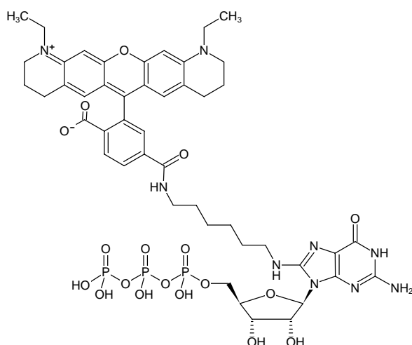
Structural formula of 8-(6-Aminoethyl)-amino-GTP-ATTO-565
