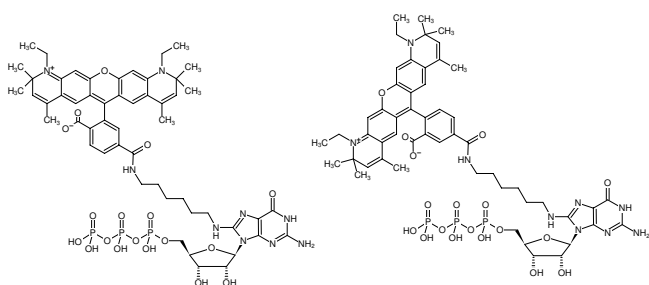
Structural formula of 8-(6-Aminoethyl)-amino-GTP-ATTO-590
