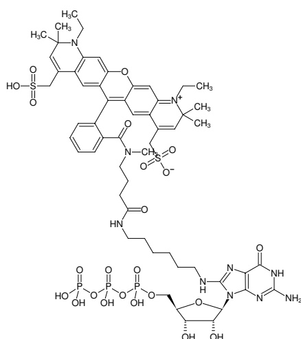
Structural formula of 8-(6-Aminoethyl)-amino-GTP-ATTO-594
