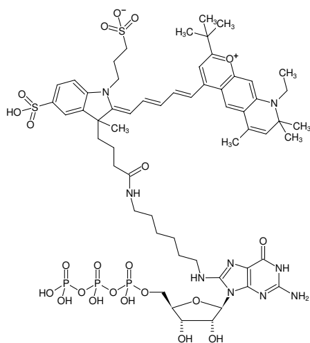
Structural formula of 8-(6-Aminoethyl)-amino-GTP-DY-751
