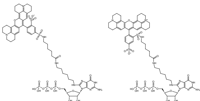
Structural formula of 8-(6-Aminohexyl)-amino-GTP-Texas Red
