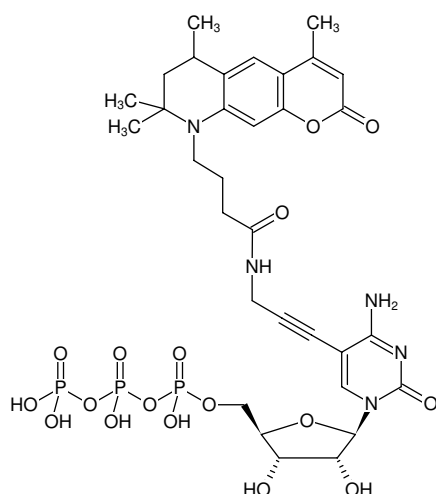
Structural formula of 5-Propargylamino-CTP-ATTO-390
