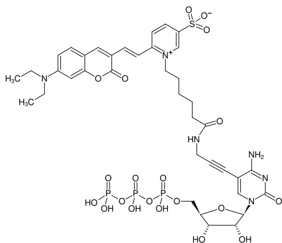
Structural formula of 5-Propargylamino-CTP-DY-480XL
