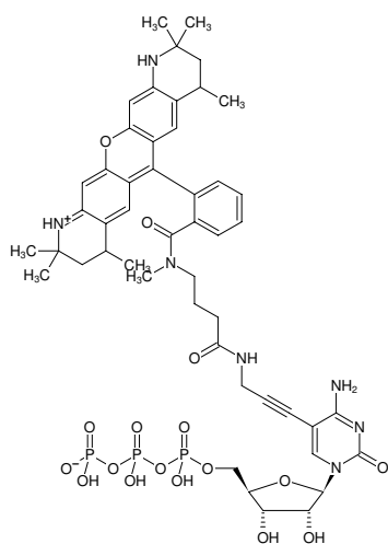
Structural formula of 5-Propargylamino-CTP-ATTO-550
