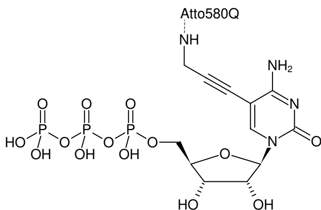
Structural formula of 5-Propargylamino-CTP-ATTO-580Q
