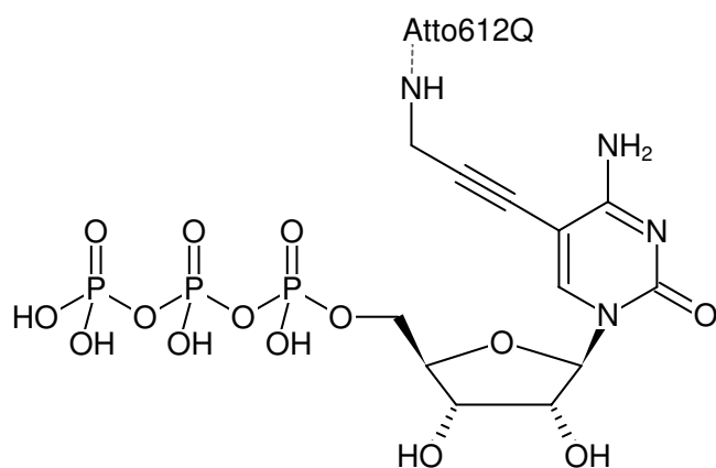
Structural formula of 5-Propargylamino-CTP-ATTO-612Q
