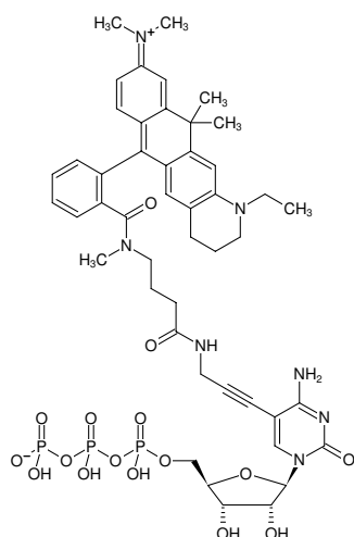
Structural formula of 5-Propargylamino-CTP-ATTO-633
