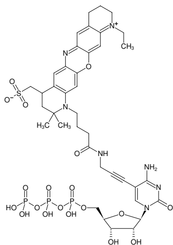
Structural formula of 5-Propargylamino-CTP-ATTO-655
