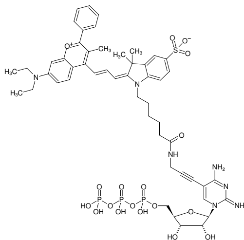
Structural formula of 5-Propargylamino-CTP-DYQ-660
