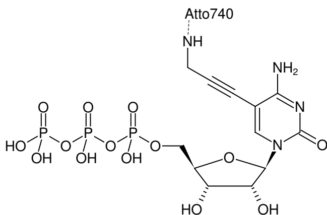
Structural formula of 5-Propargylamino-CTP-ATTO-740
