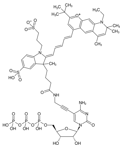
Structural formula of 5-Propargylamino-CTP-DY-751
