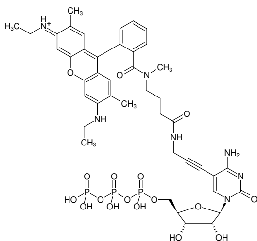
Structural formula of 5-Propargylamino-CTP-ATTO-Rho6G
