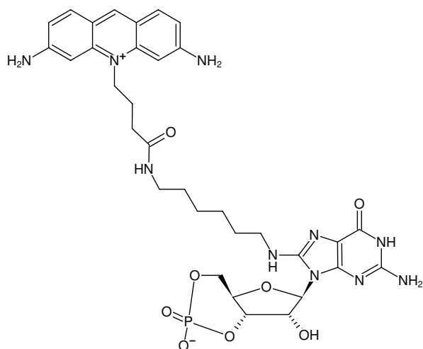
Structural formula of 8-(6-Aminoethyl)-amino-cGMP-ATTO-465
