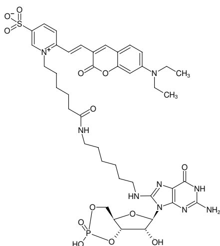
Structural formula of 8-(6-Aminoethyl)-amino-cGMP-DY-480XL
