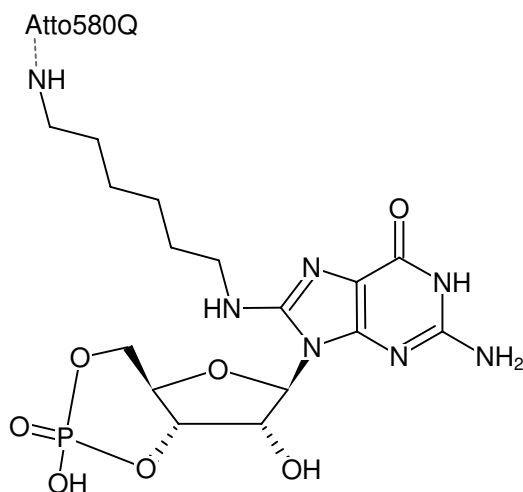
Structural formula of 8-(6-Aminoheptyl)-amino-cGMP-ATTO-580Q
