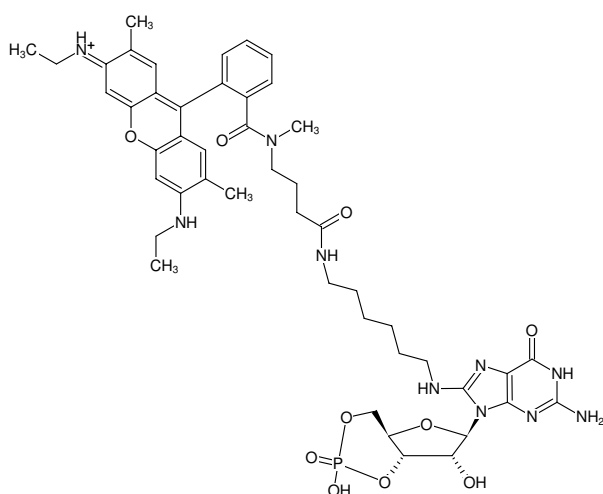
Structural formula of 8-(6-Aminoethyl)-amino-cGMP-ATTO-Rho6G
