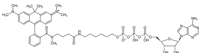
Structural formula of \gamma -(6-Aminoethyl)-ATP-ATTO-620
