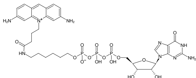
Structural formula of \gamma -(6-Aminoethyl)-GTP-ATTO-465
