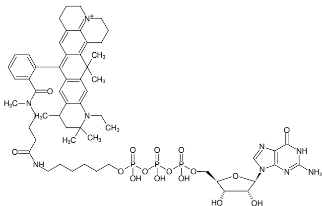
Structural formula of \gamma -(6-Aminoethyl)-GTP-ATTO-647N
