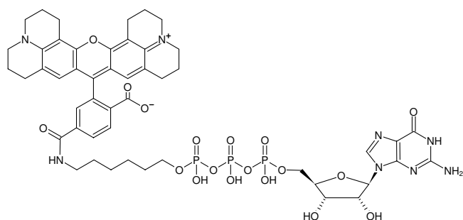
Structural formula of \gamma -(6-Aminoethyl)-GTP-6-ROX
