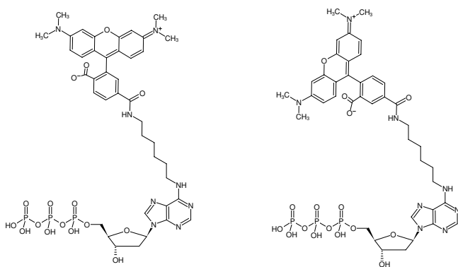
Structural formula of N 6 -(6-Aminoethyl)-dATP-5/6-TAMRA
