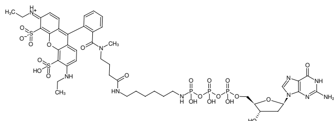
Structural formula of \gamma -[(6-Aminohexyl)-imido]-dGTP-ATTO-532
