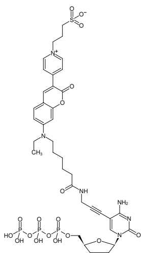
Structural formula of 5-Propargylamino-ddCTP-DY-485XL
