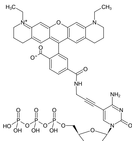
Structural formula of 5-Propargylamino-ddCTP-ATTO-565
