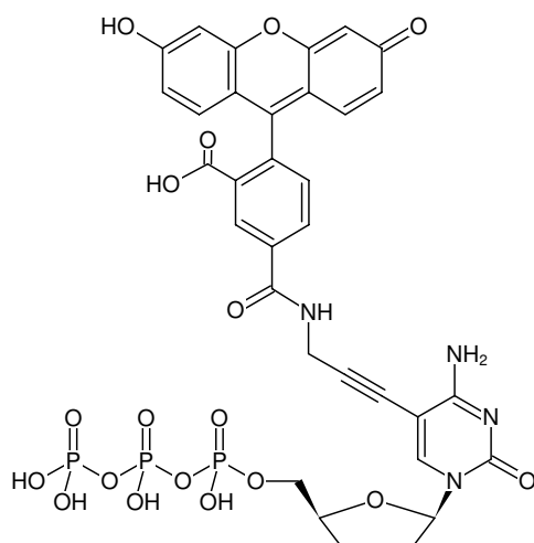
Structural formula of 5-Propargylamino-ddCTP-5-FAM
